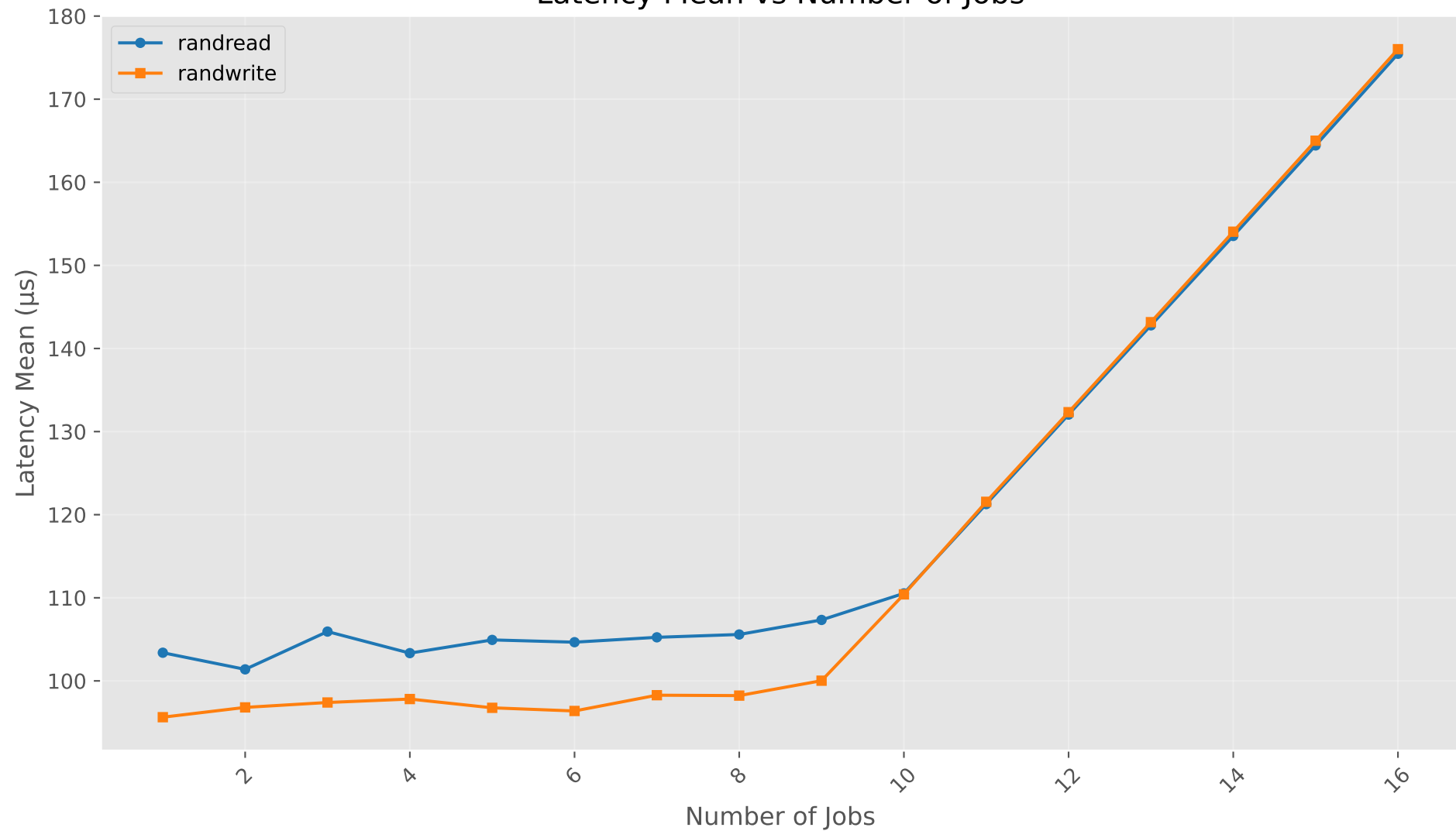
Latency Mean vs Number of Jobs
